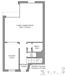
GROUND FLOOR Planta Baja
