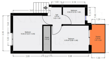
NOT TO SCALE 1st floor
