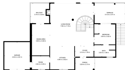
TOTAL 208 m 2 Area Constr. 181 m 2 - 100 m 2 - 118 m 2 EXCLUDED AREA: STAIRS, SET-BACK, TERRACE, BALCONY, GARAGE, TERRACE TERRACE: 17 m 2 - 102 m 2 - 87 m 2 - 100 m 2 - 118 m 2
