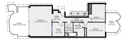
NOT TO SCALE Ground floor
