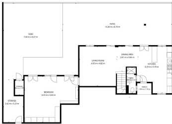
TOTAL: 113 m 2 1st Floor: 89 m 2 ; 2nd Floor: 24 m 2 EXCLUDED AREA: STORAGE: 11 m 2 ; TERRACE: 14 m 2 ; PATIO: 81 m 2 WALLS: 16 m 2
